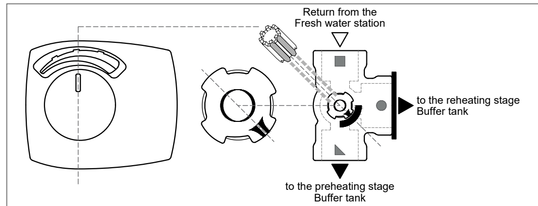
Figure 2: Installation position of the 3-way changeover valve VRG.../ARA645
